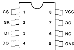
8-Pin SOIC
