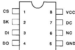
8-Pin PDIP
